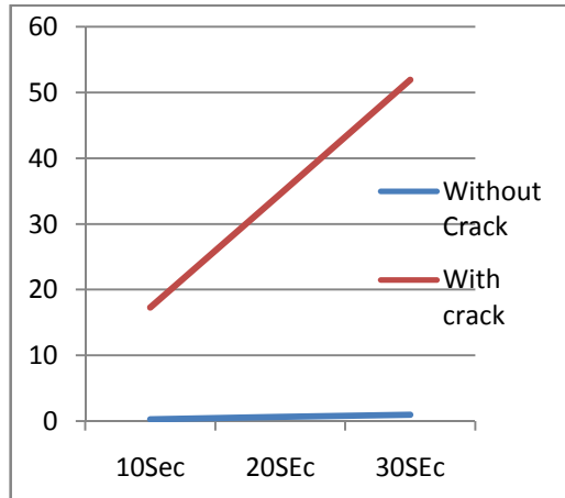
Fig 6 Graphical representation of stress values of dynamic analysis – without crack and with crack ( a) aluminum 7475 (b) aluminum 6061 (c) s2 glass (d) kevlar
